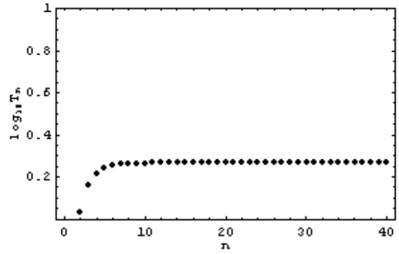
Fig. 4 time required to conduct computation at each step by using superluminal particles (for the case, k = 1/2 and \gamma = 1.0 ).
