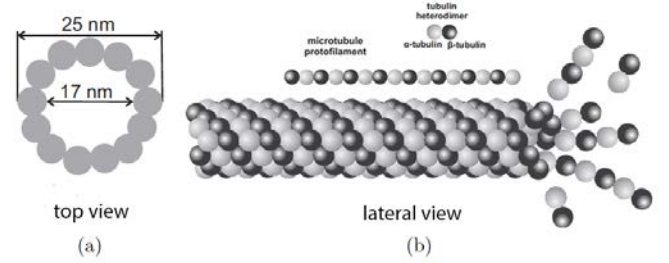
Fig. 1 schematic view of MT structure and its constituents
