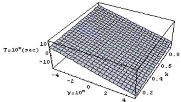
Fig. 5 computational required time for the superluminal particles.
