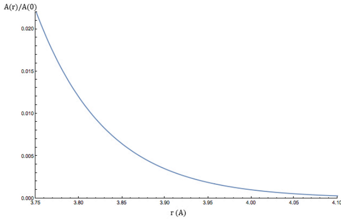
Fig. 2 tail of coherent electromagnetic field of a water CD
