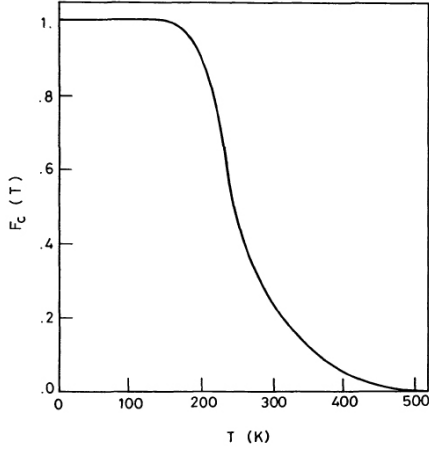
Fig. 3 behavior of coherent fraction in water [28,33]
